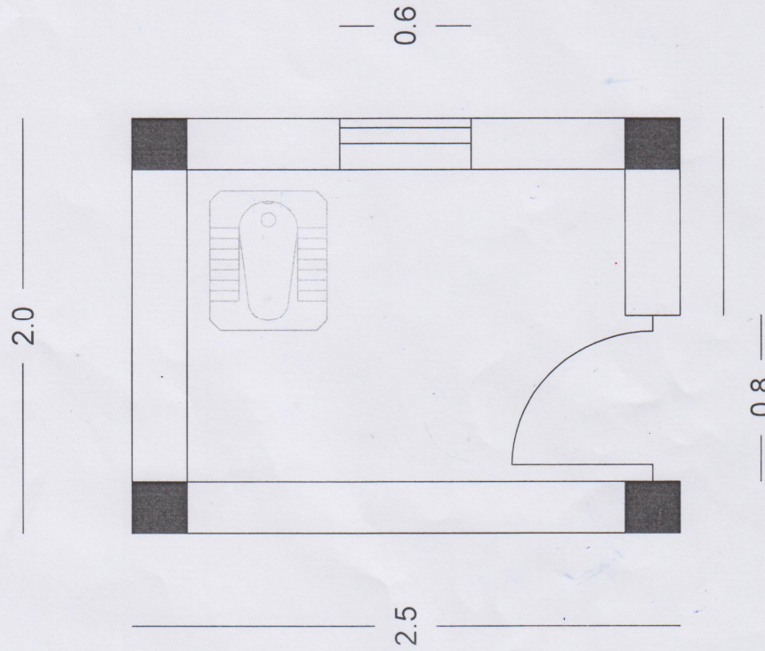
Plan of Bathroom
