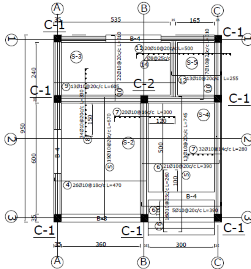
Reinforcement Plan
