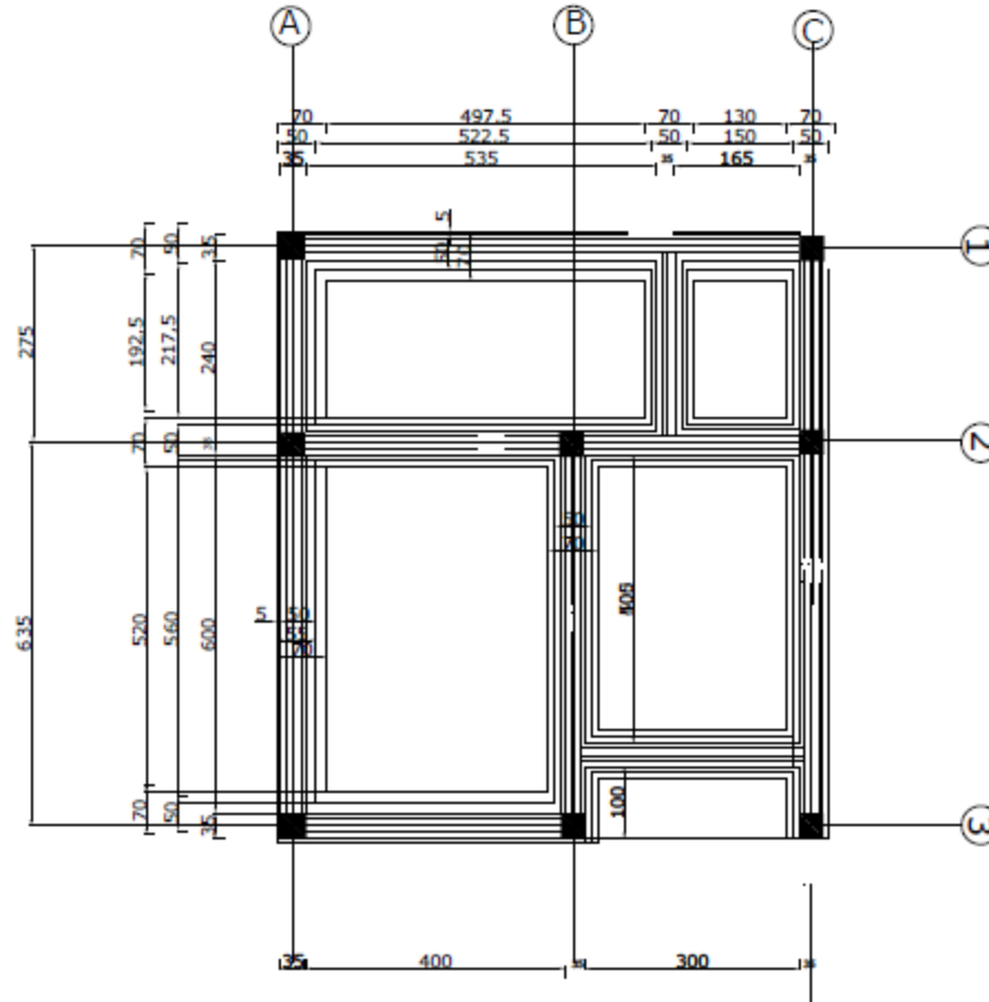
Foundation Plan
