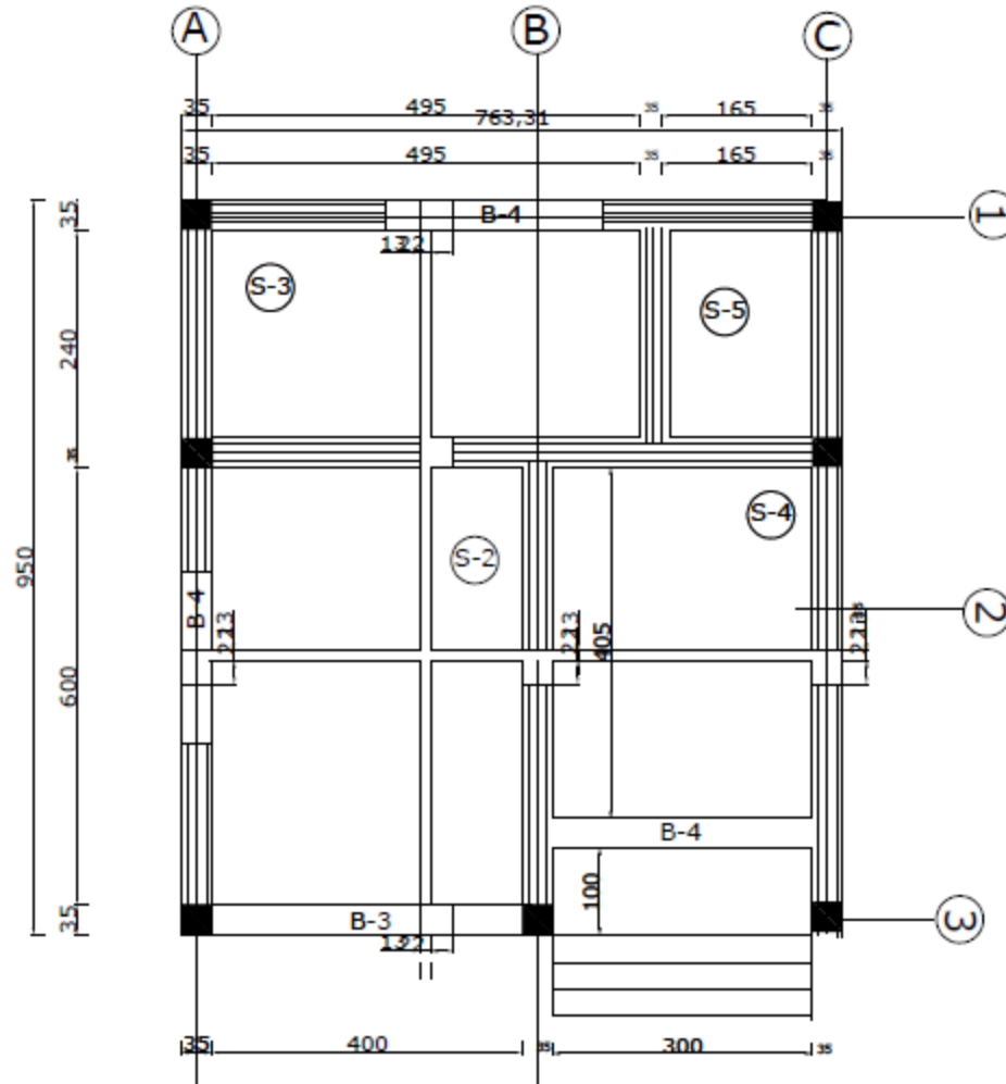
shuterling Plan
