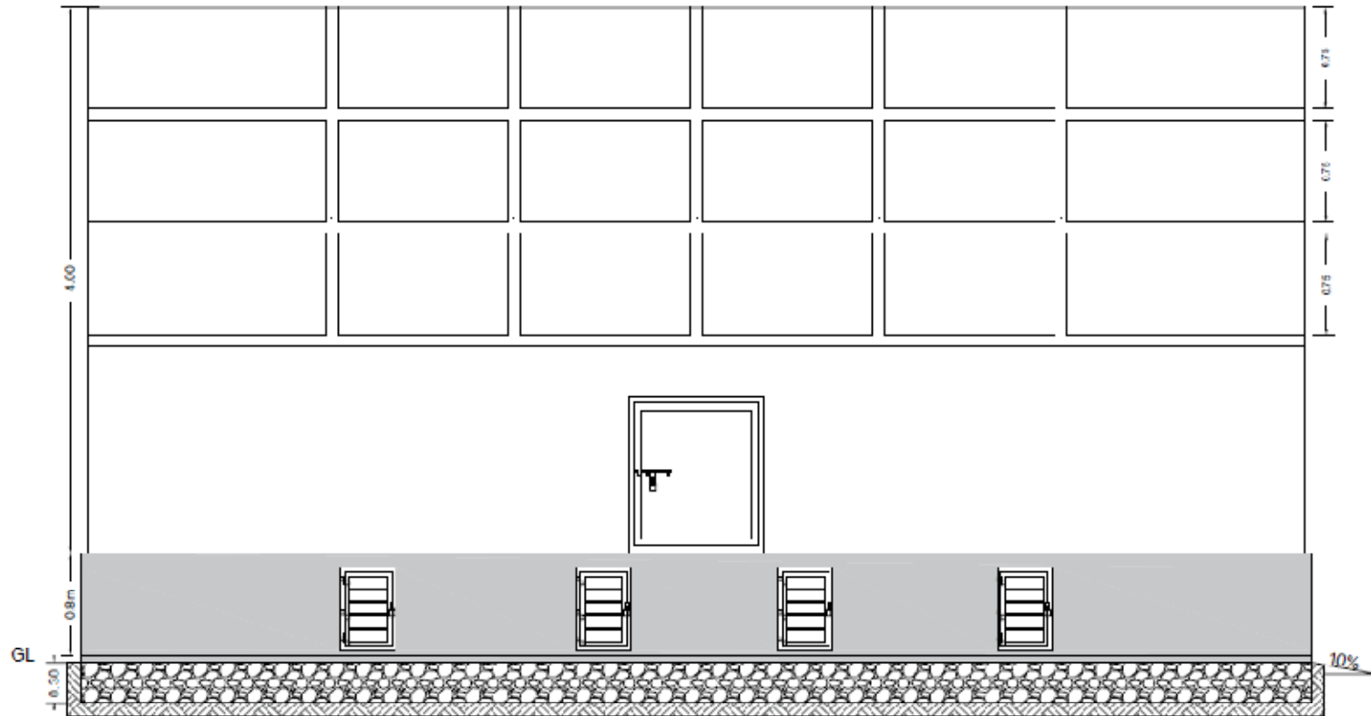
Rectangular furnace Front View
