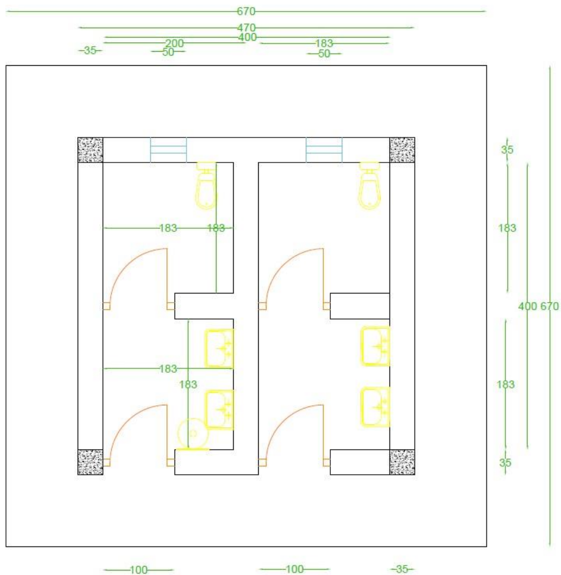
bath room plan
