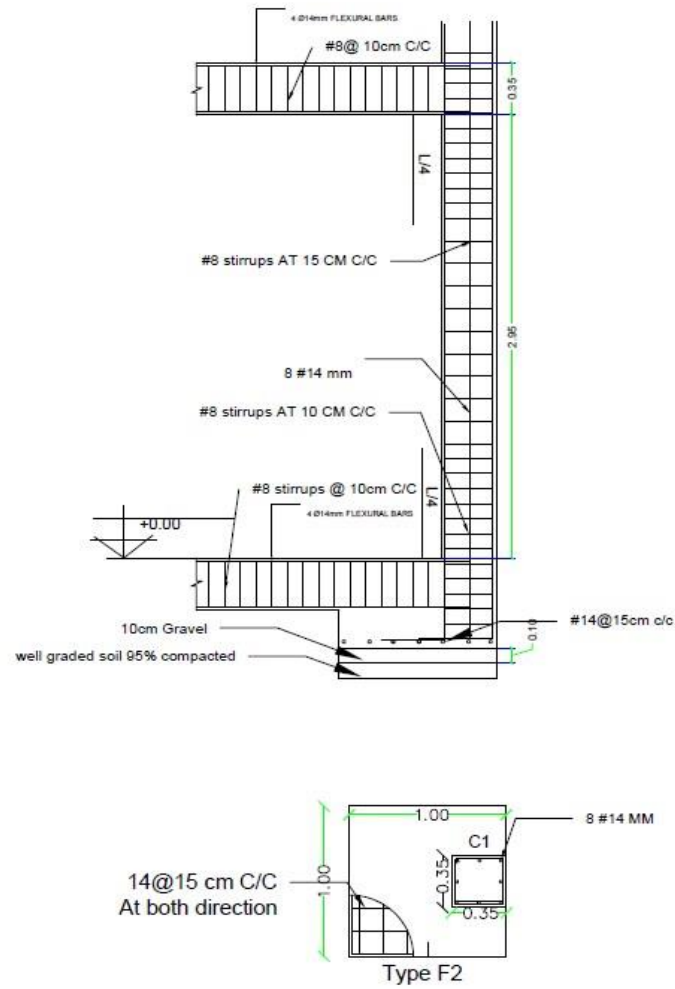
Column Plan Detail Scale:1:50
