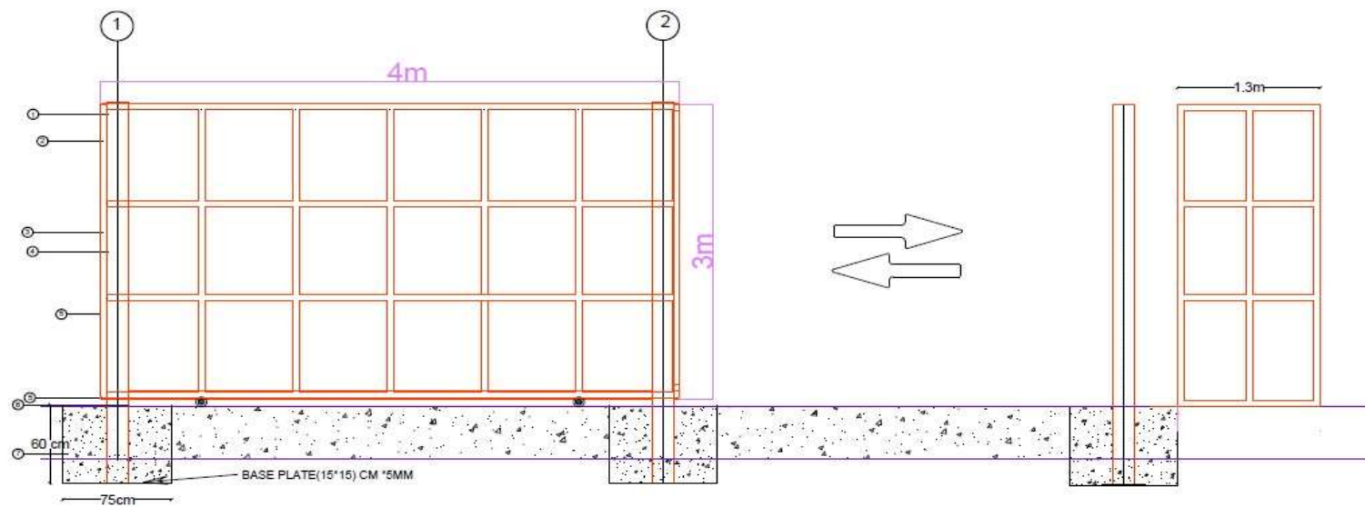
PROFILE PLAN
