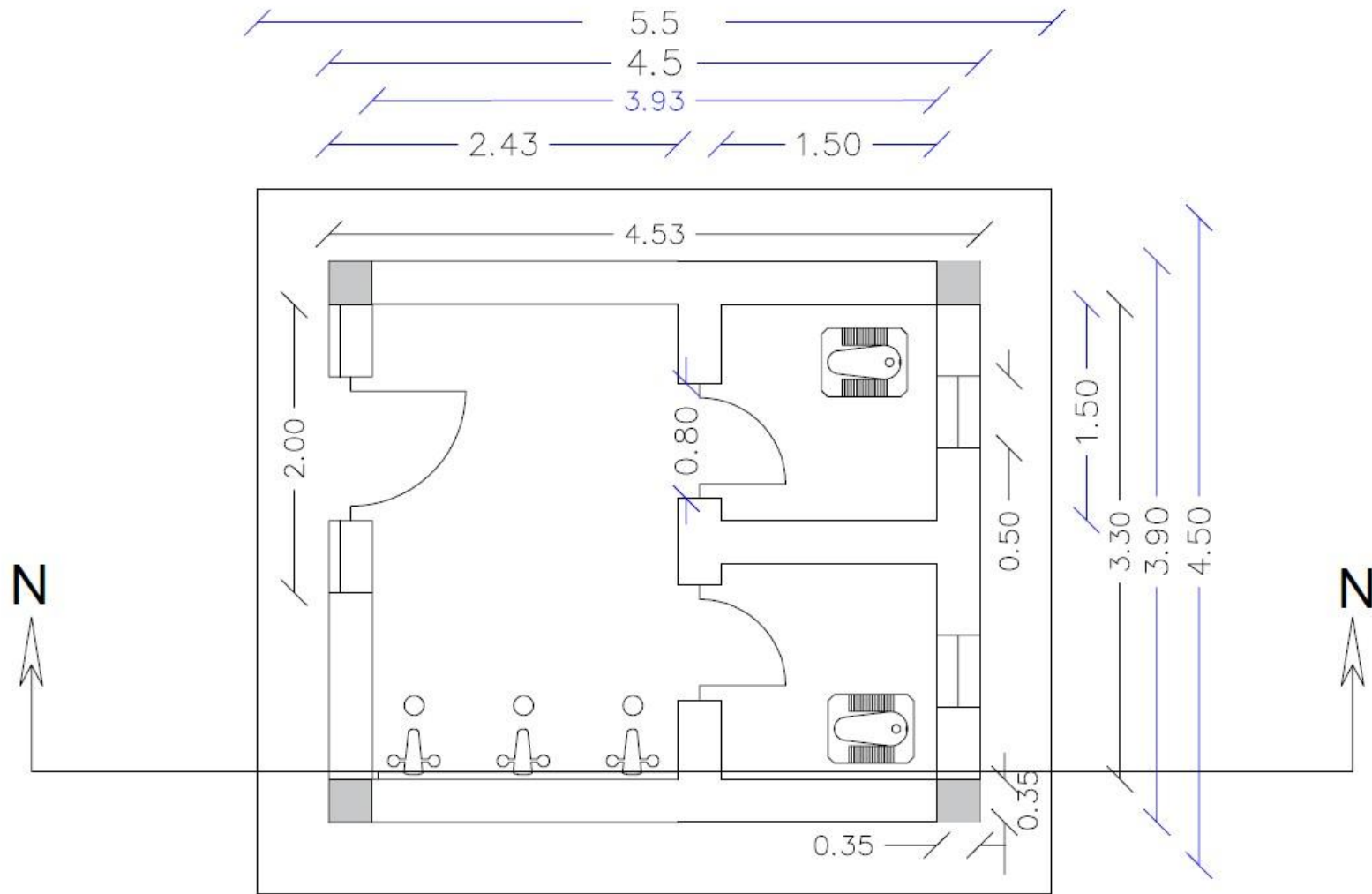
Ablution area plan
