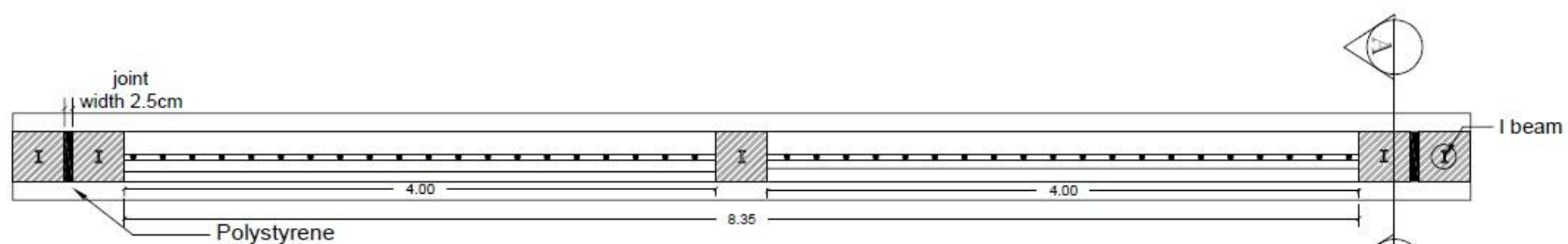
Top view
