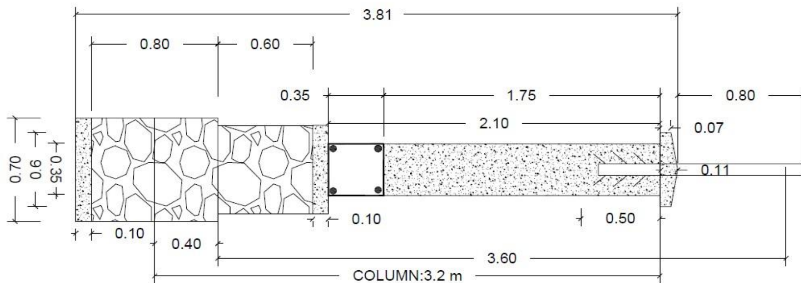
section
