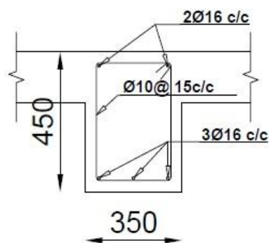
Section 2
