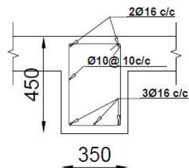
Section 1
